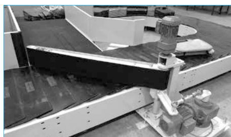
Soft horizontal diverter
